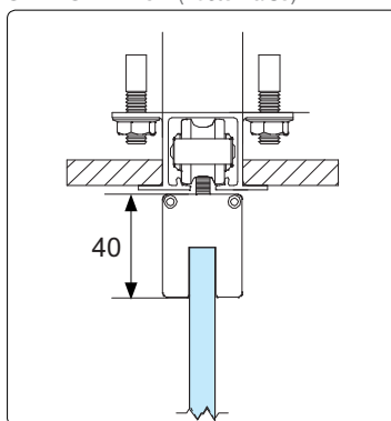
SV-EASY LARGE (Tecto Falso)
